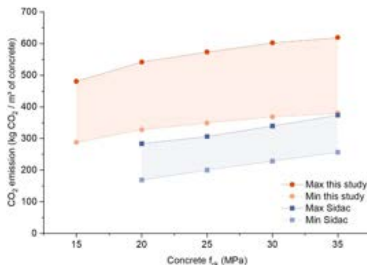
Figure 8. CO 2 emissions for concretes of different grades produced in Acre calculated using the methodology developed in the study in comparison with CO 2 emissions for similar concretes available in the Sidac database.
