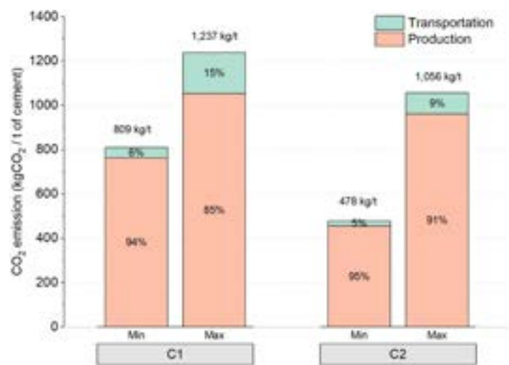
Figure 4. Minimum and maximum CO 2 emissions of cements considered in this study.
